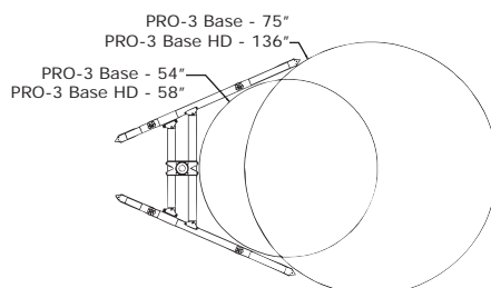
Pt#30189 PRO-3 Base, External Tank Collar (3 piece) Grip range 3/16" to 3 1/4"
